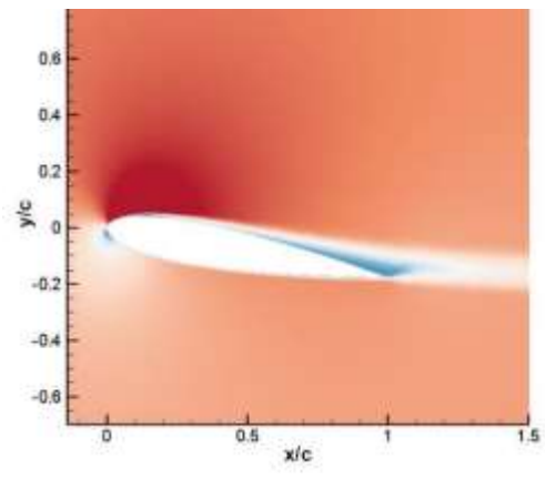
AoA=10°
