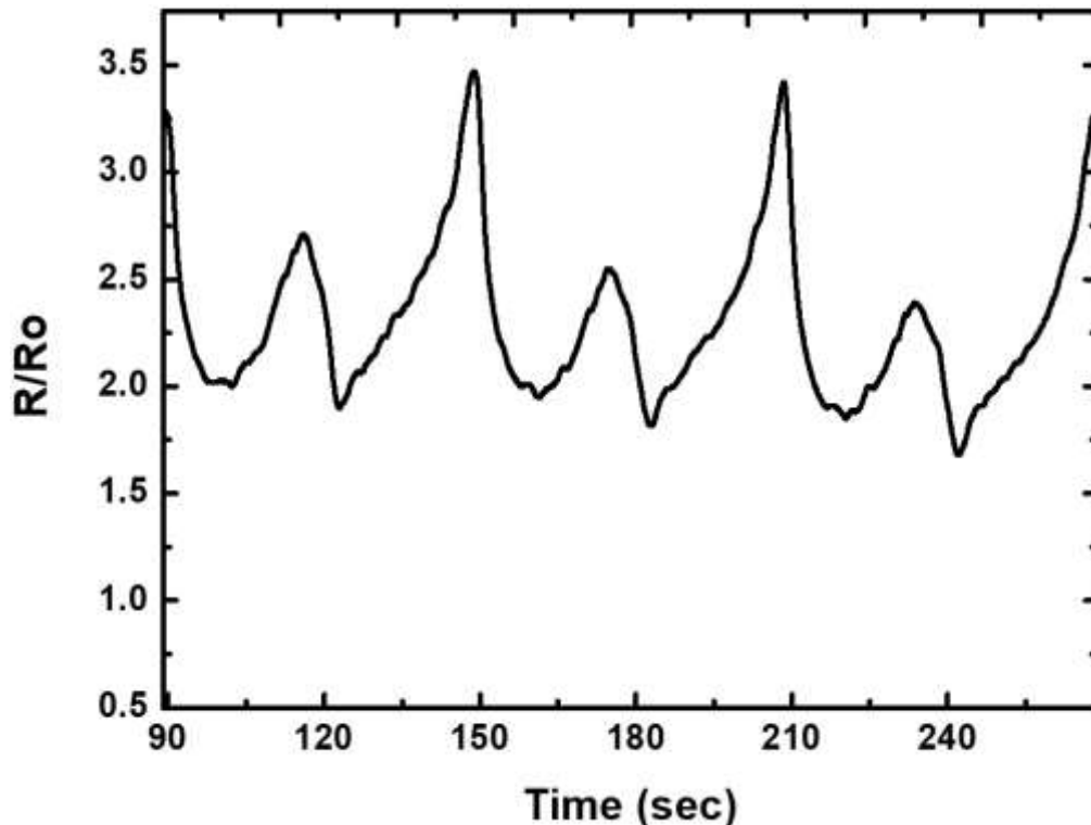
Figure 4. 3 rd -5 th cycles for piezoresistive sensing of 30/70 PBC/SEBS flexible composite
