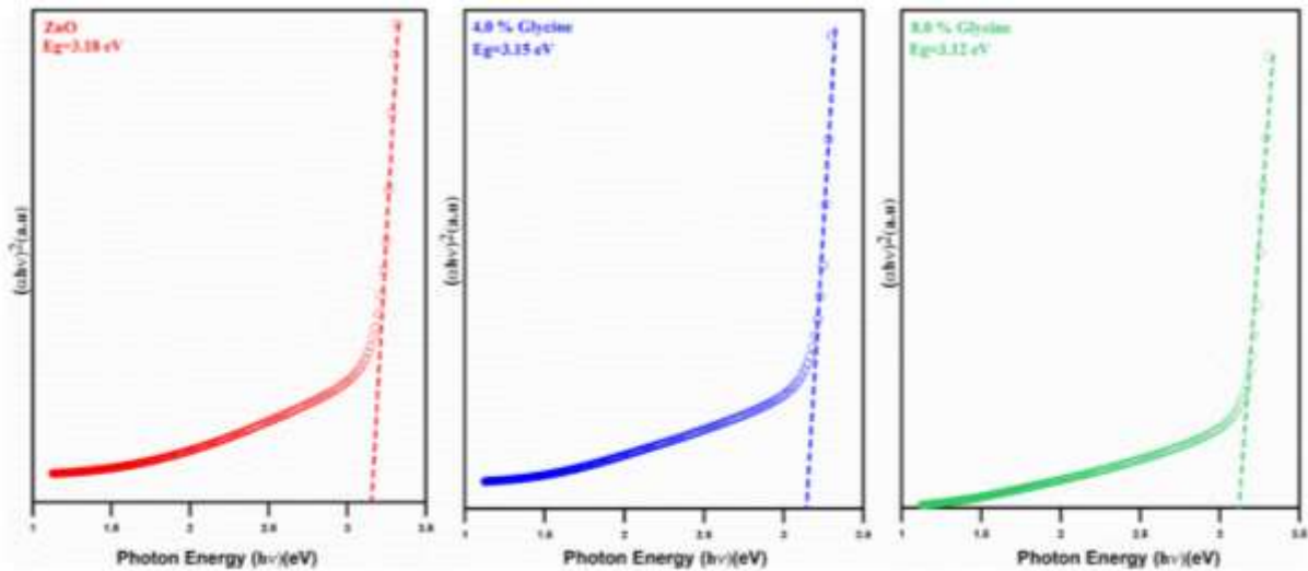
Figure 5. Tauc's plot of deposited ZnO films with different glycine content.
