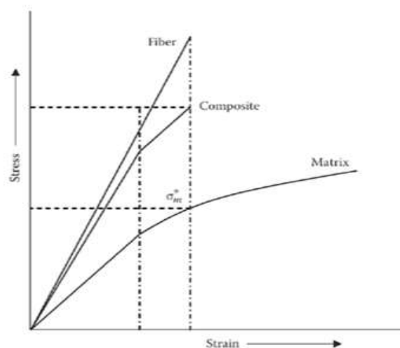
Fig.3 Stress-strain plot for fiber-reinforced composites
