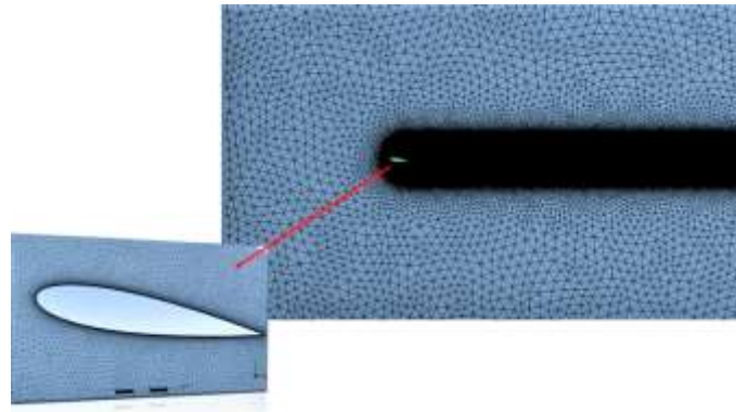
Figure 2. The mesh structure on NACA0015 airfoil
