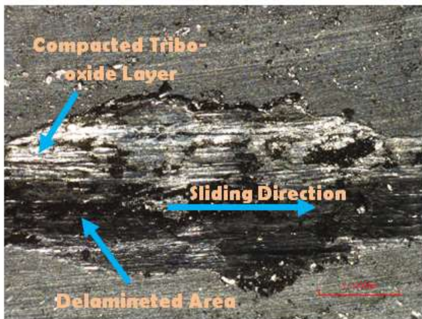
Figure 4. Wear print of after extrusion of Al6063 Alloy.
