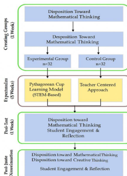
Figure 3. Experimental Design
