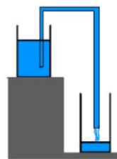
Figure 1. Pythagorean Cup
